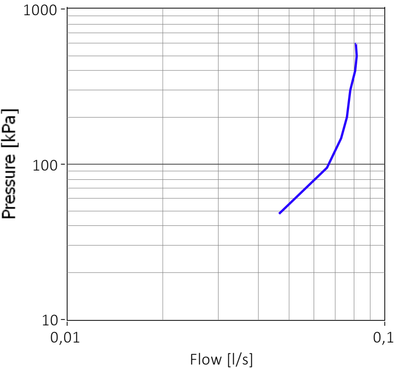
FLOWCHART AS A FUNCTION OF INLET PRESSURE
